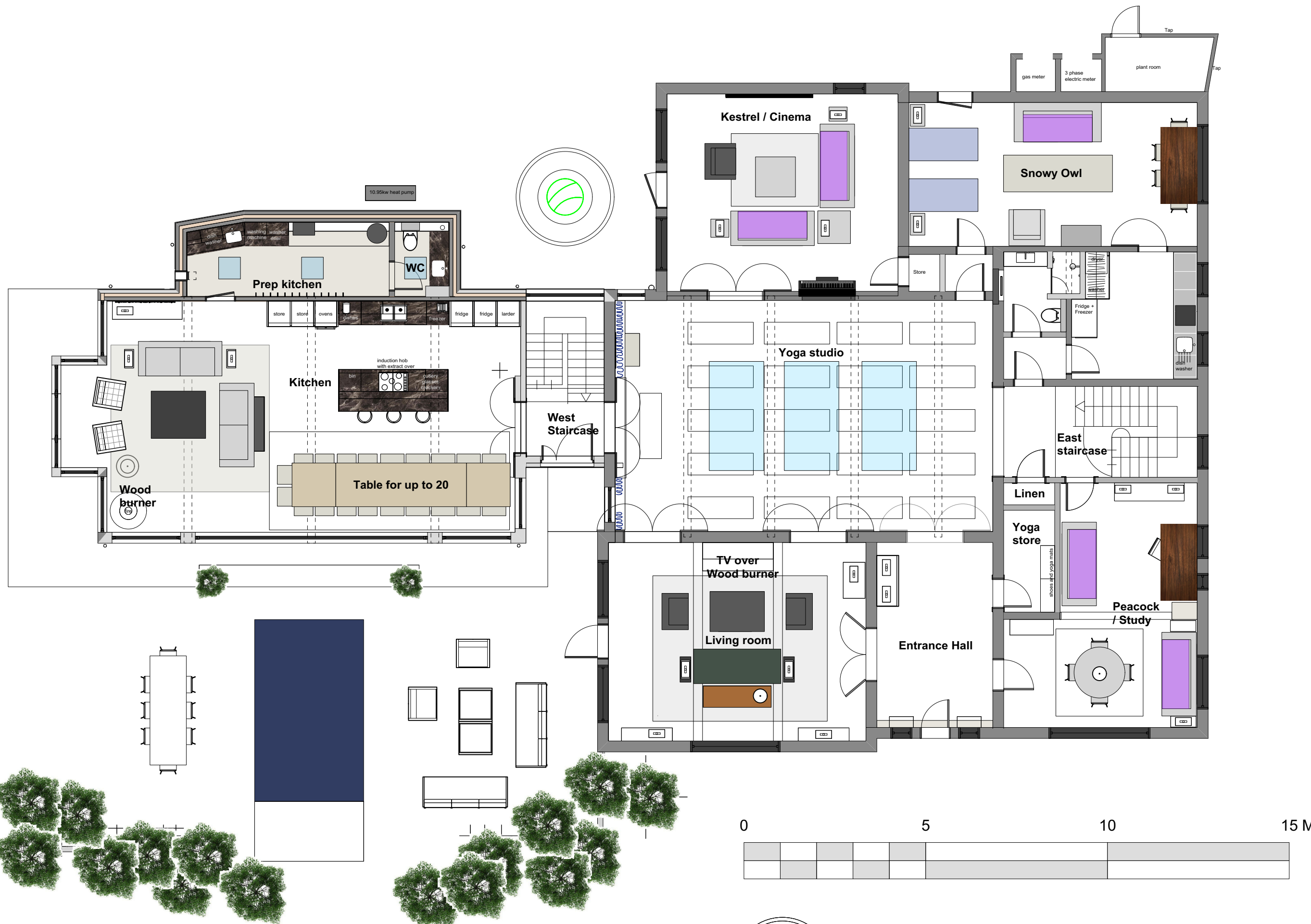
RIVERSDALE LODGE R 003 R1 GROUND FLOOR PLAN 1:100 ON A3 DRAWN 4.1.2023 ZODIAC DESIGN
